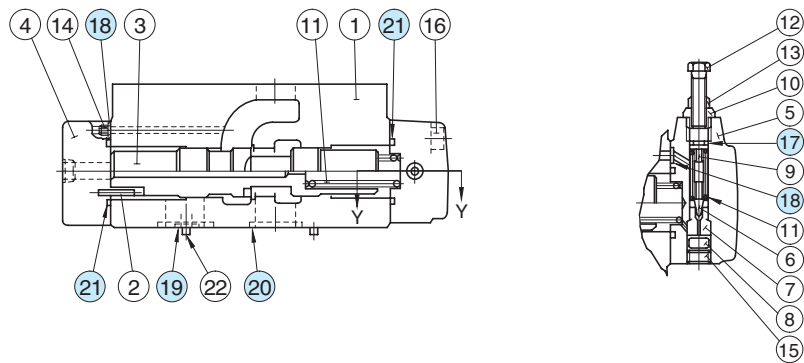
Section Y-Y
