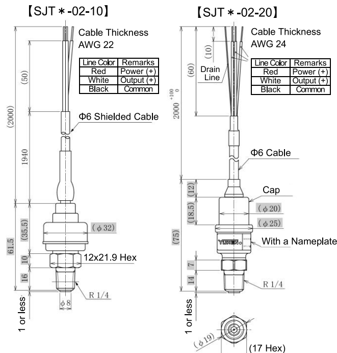
Fig.1 External Dimensions
