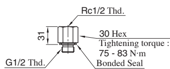
Adapter
