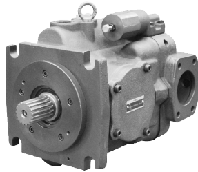
A3HG 系列高压变量柱塞泵 “A3HG” Series High Pressure Variable Displacement Piston Pumps
