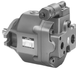
AR 系列变量柱塞泵 “AR” Series Variable Displacement Piston Pumps
